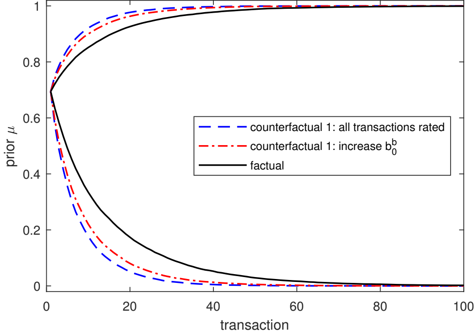
Notes: Evolution of the prior for a high- and a low-quality seller in two counterfactual scenarios. Average across 10,000 simulation runs. In scenario 1, all transactions are rated. In scenario 2, the baseline probability to rate is the same for good and bad experiences. Based on setup and procedure described in Section 7.1 and parameter values in Section 7.3.
